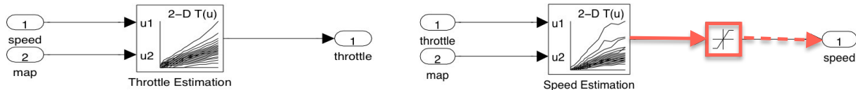
Figure 3. A type 3 (near-miss) model clone - the Throttle.throttle_estimate subsystem (Left) and Speed.speed_estimate subsystem (Right) of the sldemo_fuelsys model. NiCad similarity 66%
