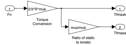
Figure 1. A type 1 (exact) model clone - the Friction Mode subsystem, which occurs in both the Sldemo_Clutch and the Sldemo_Clutch_if example models. NiCad similarity 100%
