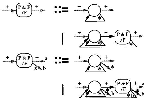
Fig. 15. Pipe and filter system with feedback.
