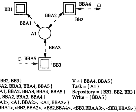
Fig. 9. Example translation of a subsystem.
