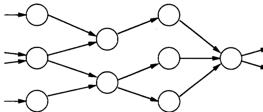
Fig. 16. Example pipe and filter system.
