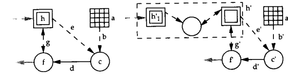
Fig. 11. Example pattern match.
