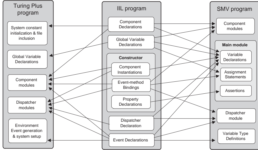
Figure 5. Diagram showing how the parts of an IIL program are used in generating the corresponding Turing Plus program and SMV model
