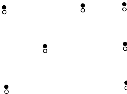
Figure 3. The construction of T .
