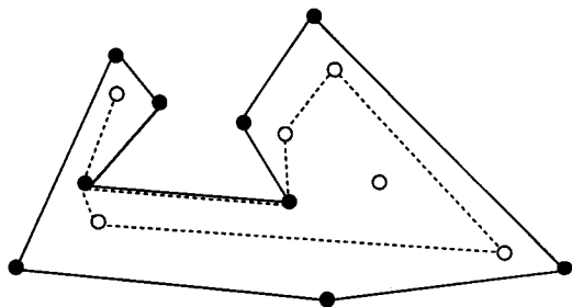
Figure 2. CH(S|T) is denoted by dashed lines.
