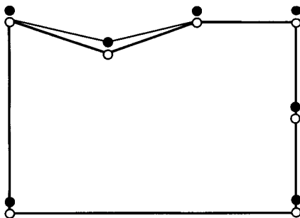
Figure 4. We replace two edges in the polygon P to create the travelling salesman tour \bar{Q} and increase the total length by no more than 2\epsilon .
