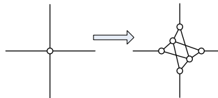
Figure 4: Transformation of a degree 4 vertex of the input graph according to Umans' algorithm [12].
