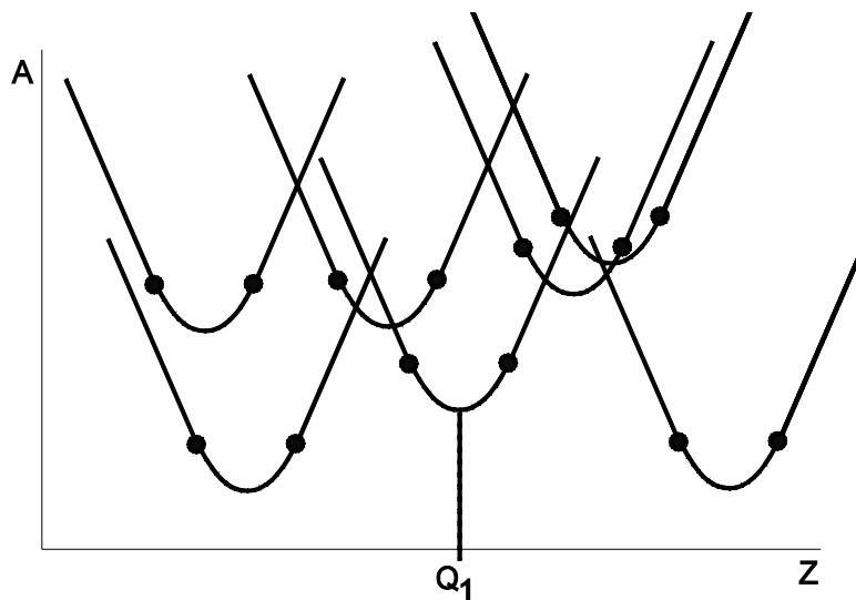
Figure 6: The median Q_1 of function minima.
