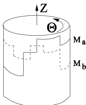
Figure 2: Two orthogonal periodic melodies.
