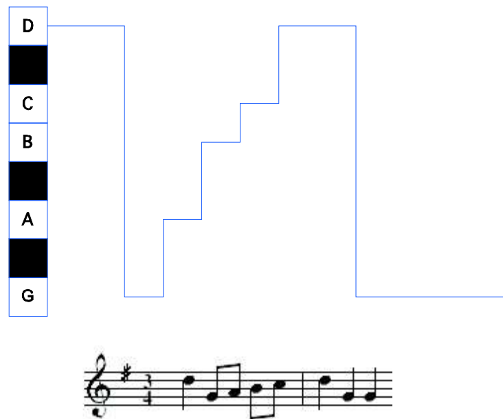
Figure 1: The first two measures of a well known melody are shown below our representation using an orthogonal polygonal chain.
