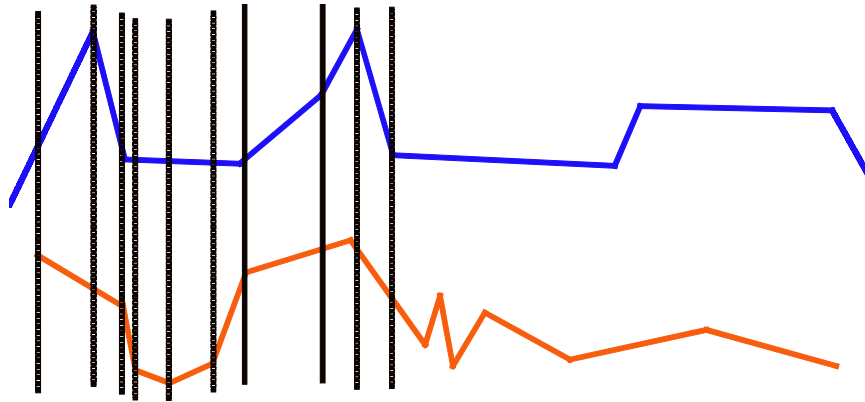
Figure 4: Two monotone chains and their strips.
