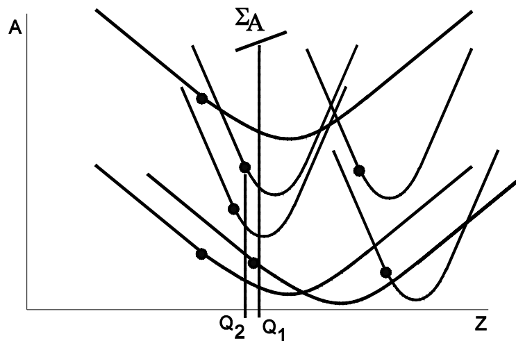
Figure 8: Q_2 to the left of Q_1 .
