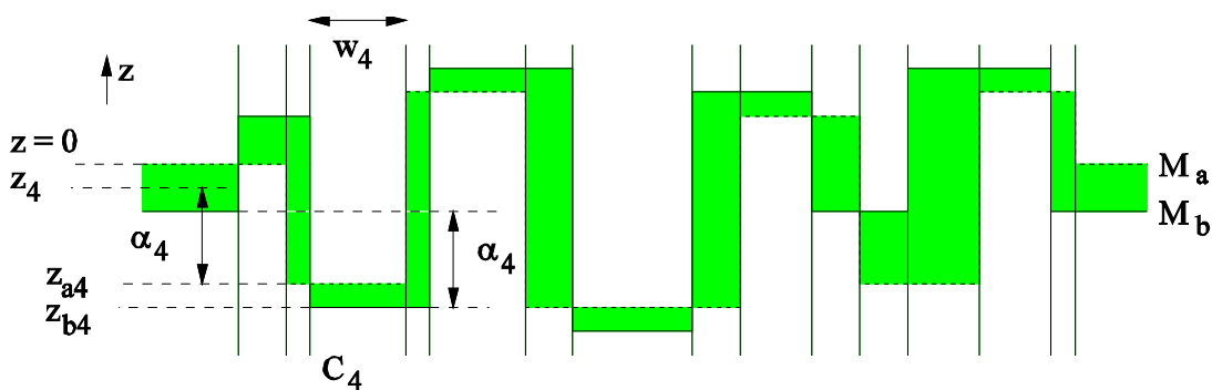
Figure 3: Contribution of C_4 to area calculation.
