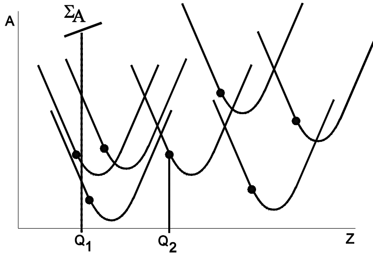
Figure 7: The median Q_2 of left inflection points.
